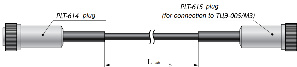
Figure A.5 – Measuring cable КИ-ИТСВ
